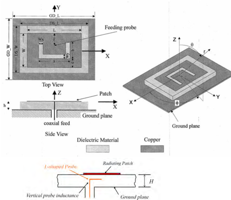
Figure 28.11: The top figure shows a U slot patch antenna design. The bottom figure shows a patch antenna fed by an L probe with significant increase in bandwidth (courtesy of K.M. Luk) [156].
