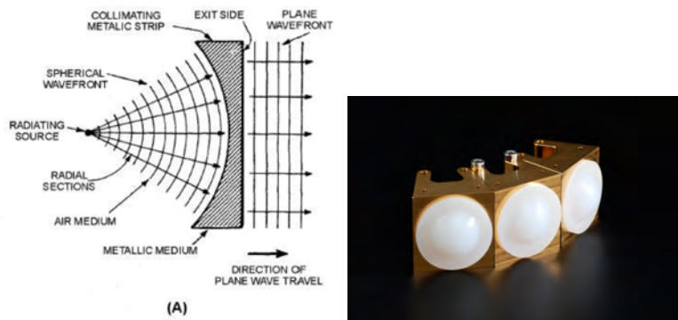
Figure 28.9: The left figure shows a lens antenna where the lens is made of artificial dielectrics made from metallic strips (courtesy of electriciantutoring.tpub.com). The right figure shows some dielectric lens at the aperture of an open waveguide to focus the microwave exiting from the waveguide opening (courtesy of micro-radar.de).
