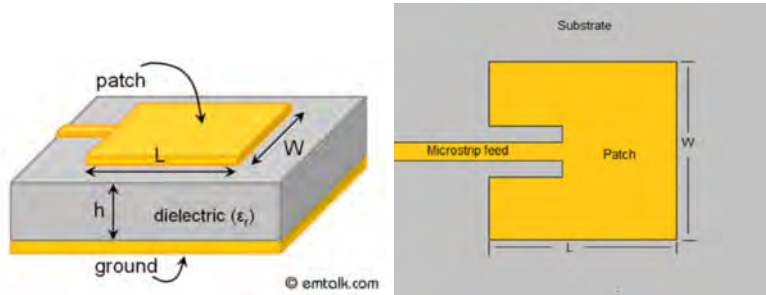
Figure 28.4: A microstrip patch antenna also radiates well when it resonates. The patch antenna resembles a cavity resonator with magnetic wall (courtesy of emtalk.com).
