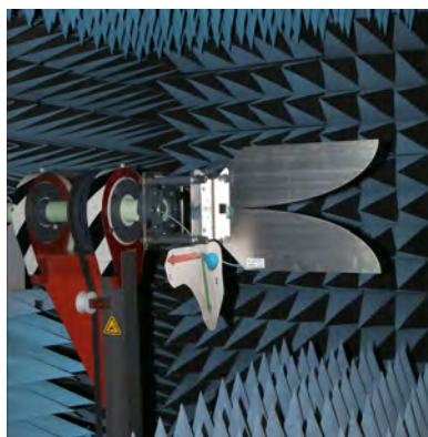
Figure 28.6: A Vivaldi antenna, also called a notch antenna, works like a horn antenna, but uses very little metal. Hence, it is cheap to build, and its flared notch makes it broadband (courtesy of Wikipedia [144]).
