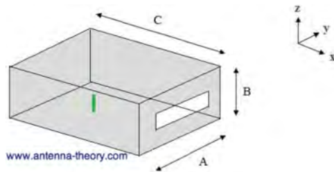
Figure 28.3: A cavity-backed slot antenna radiates well because when the small dipole radiates close to the resonant frequency of the cavity, the field strength is strongly enhanced inside the cavity, and hence around the slot. This makes the slot into a good radiator (courtesy of antenna-theory.com).
