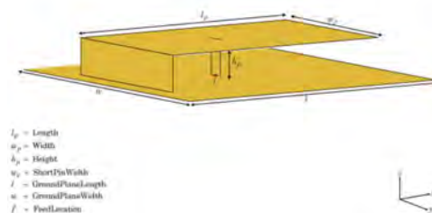
Figure 28.10: A PIFA (planar inverted F antenna) is compact, broadband, and easy to fabricate. It is good for cell phone antennas due to its small size (courtesy of Mathworks).
